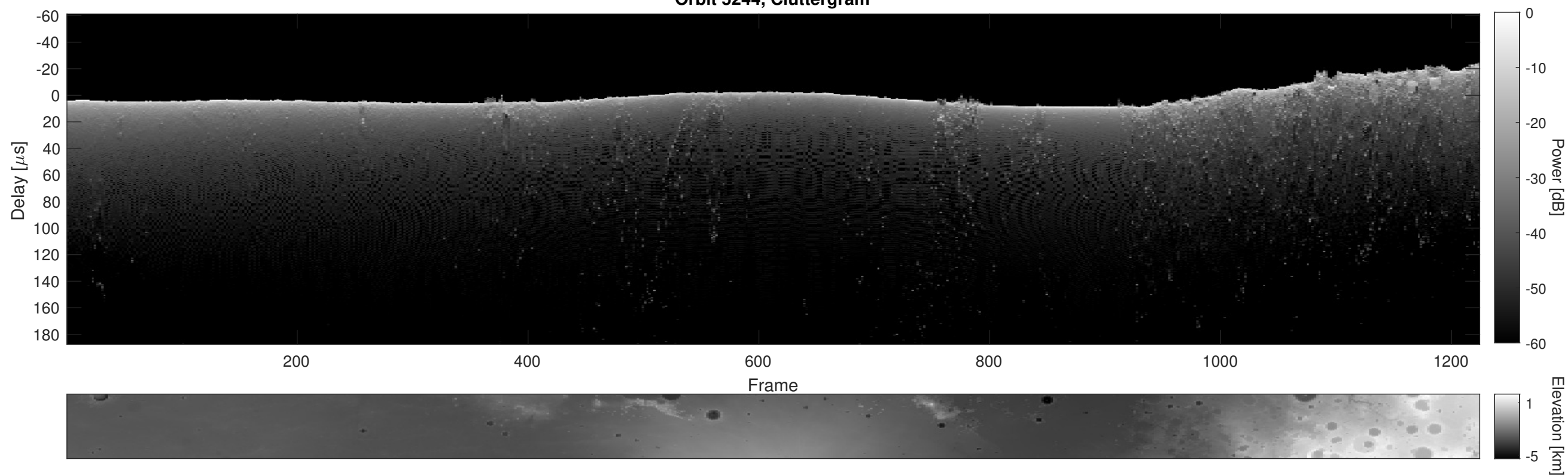
Orbit 5244, Cluttergram
