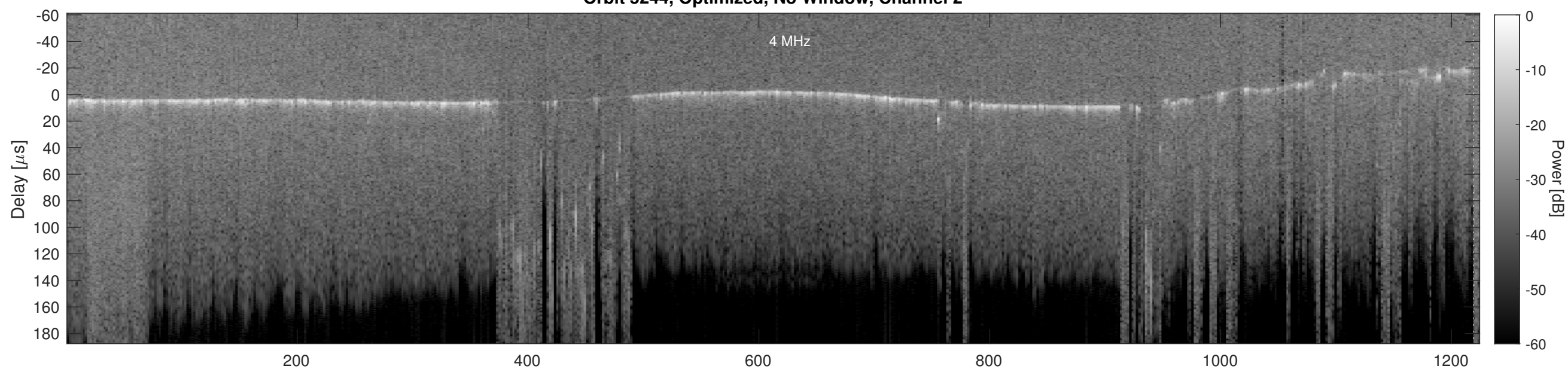
Orbit 5244, Cluttergram
