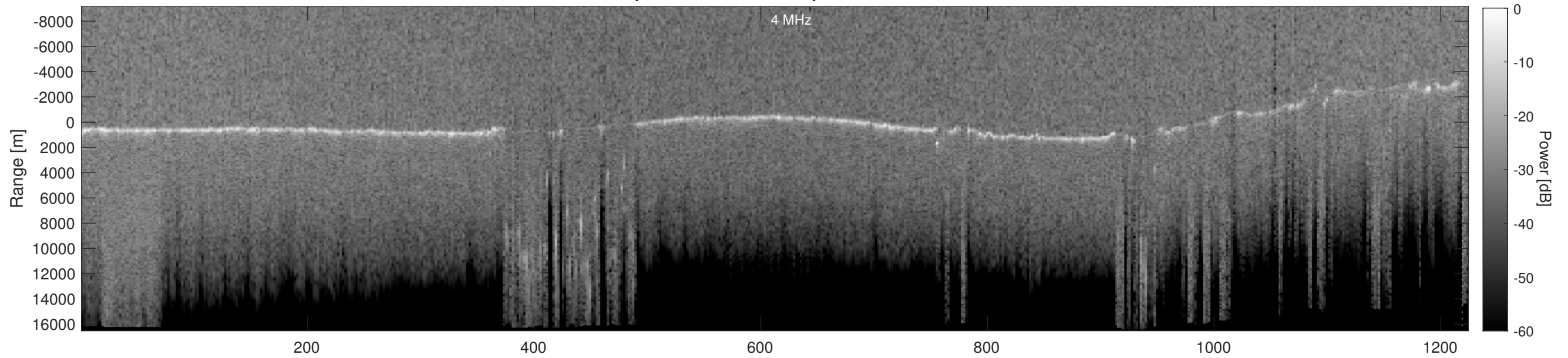
Orbit 5244, Depth-Corrected Cluttergram
