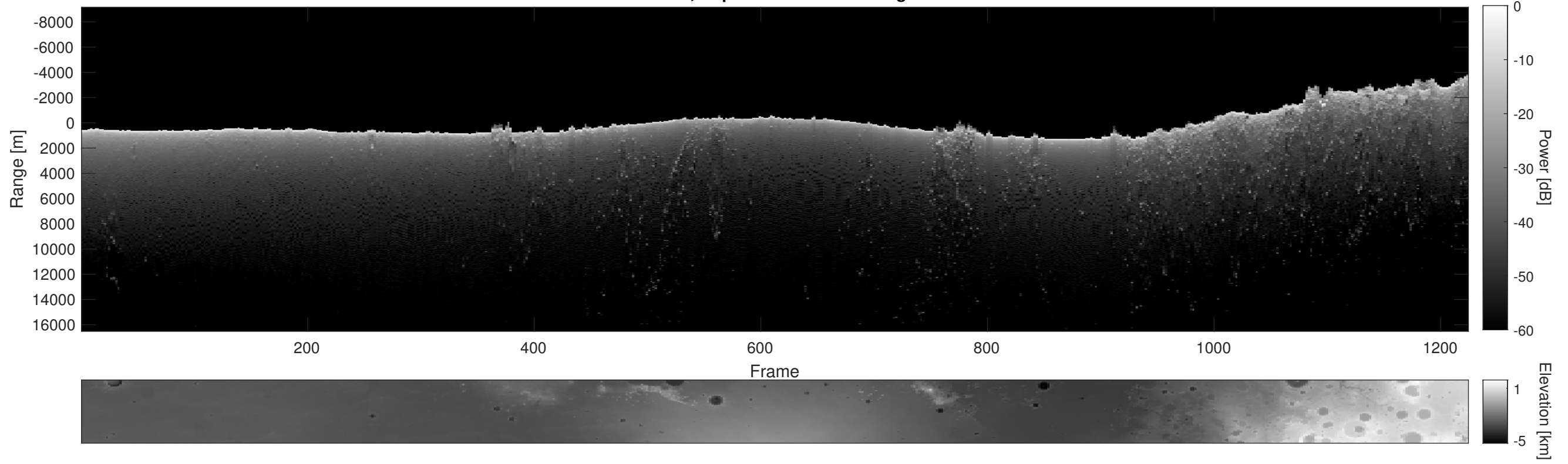
Orbit 5244, Depth-Corrected Cluttergram
