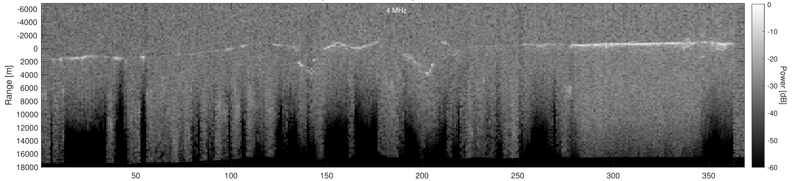
Orbit 5246, Depth-Corrected Cluttergram
