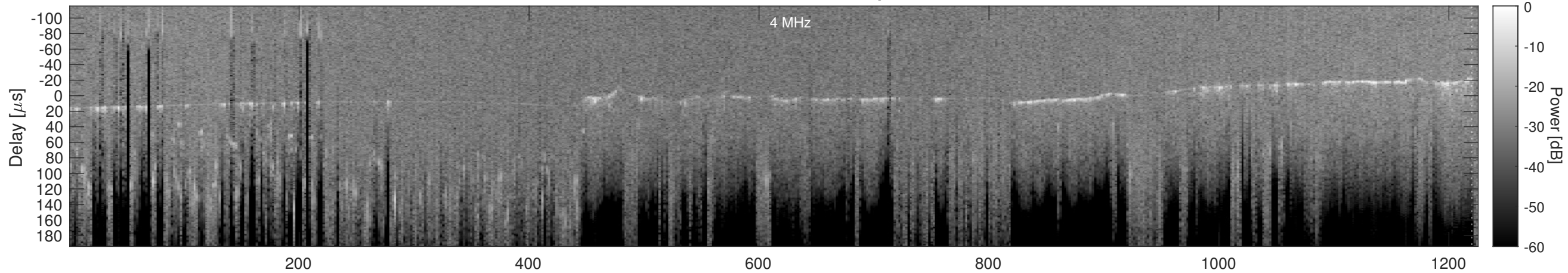
Orbit 5247, Cluttergram
