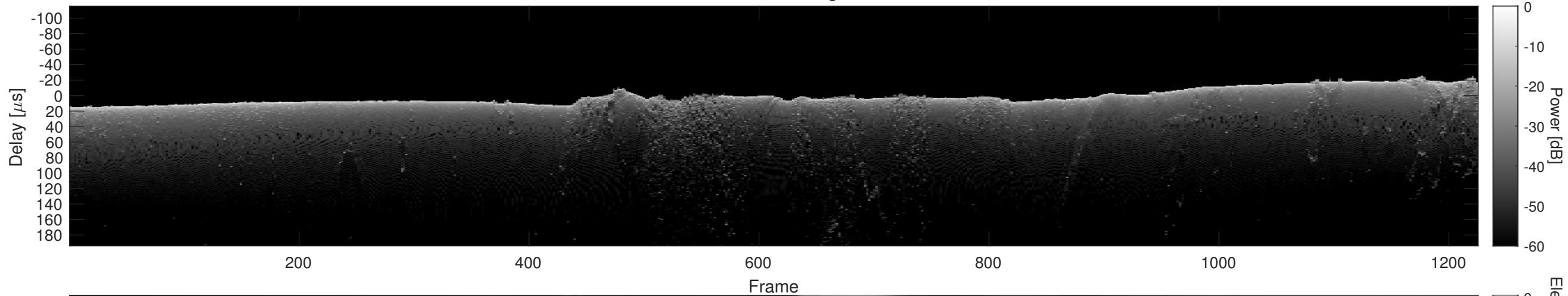
Orbit 5247, Cluttergram
