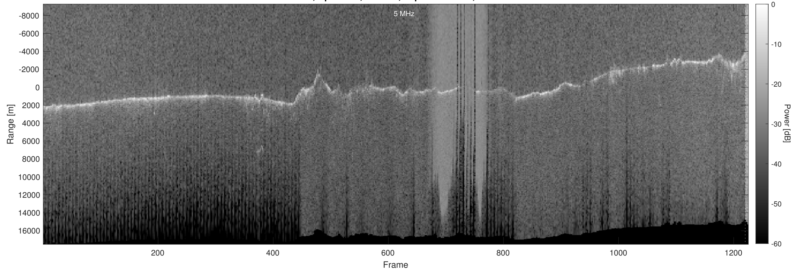
Orbit 5247, Optimized, Window, Depth-Corrected, Channel 2
