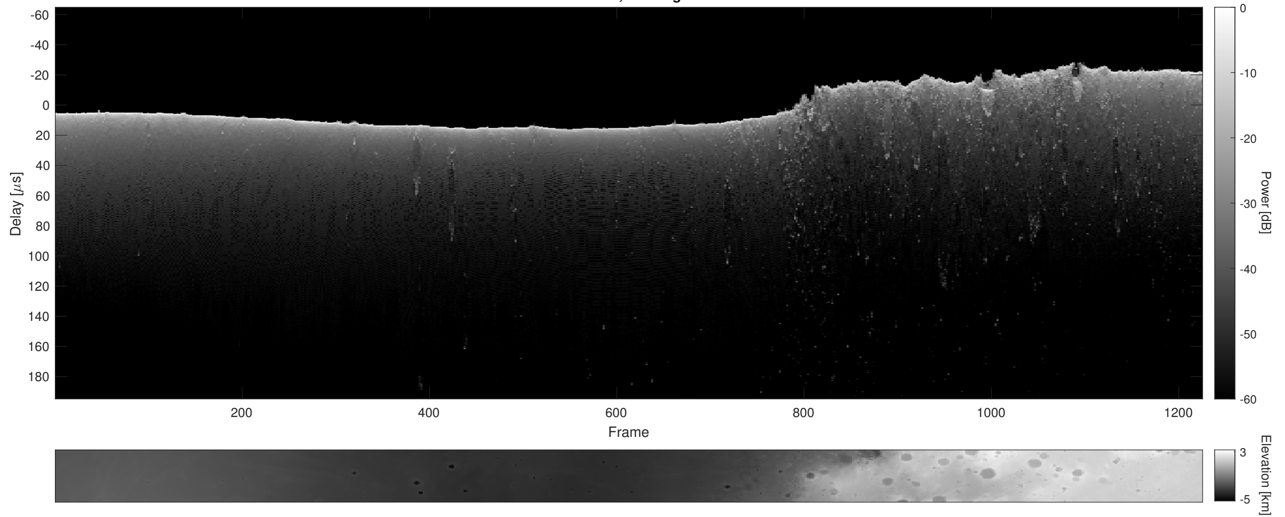
Orbit 5248, Cluttergram
