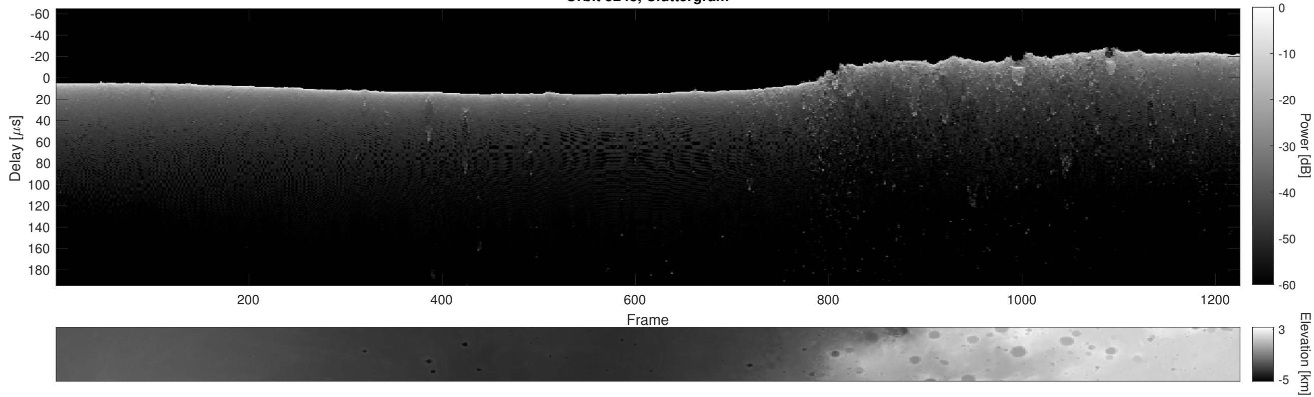
Orbit 5248, Cluttergram
