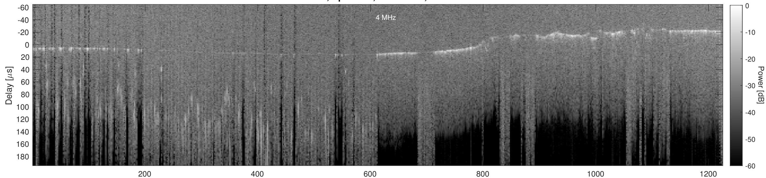
Orbit 5248, Cluttergram
