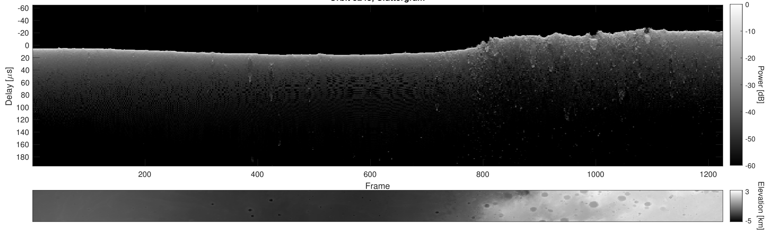
Orbit 5248, Cluttergram
