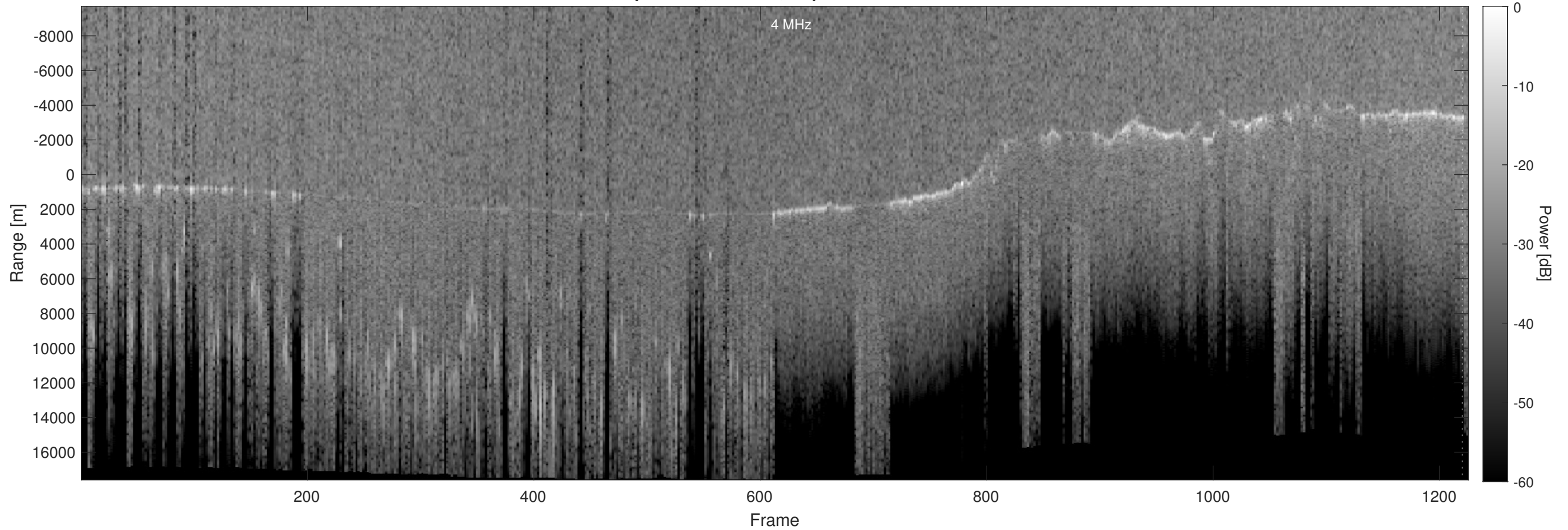
Orbit 5248, Optimized, Window, Depth-Corrected, Channel 2
