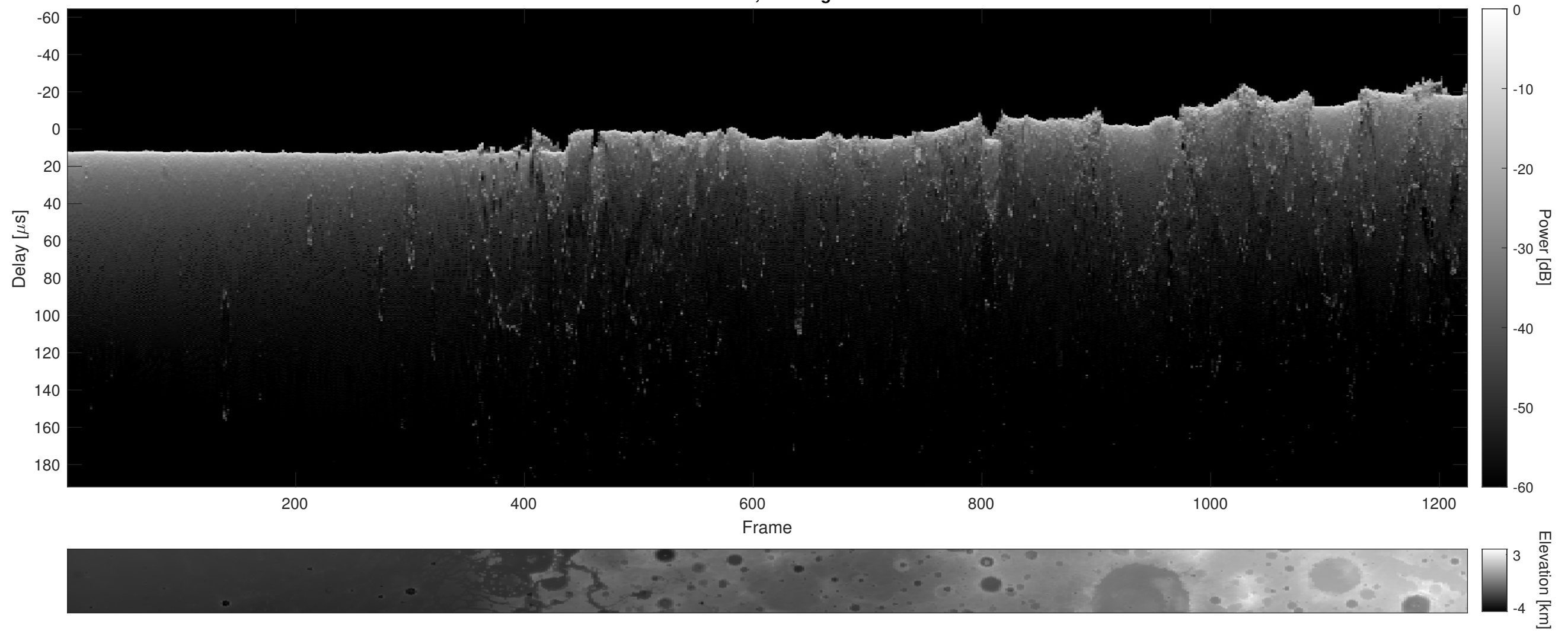
Orbit 5249, Cluttergram
