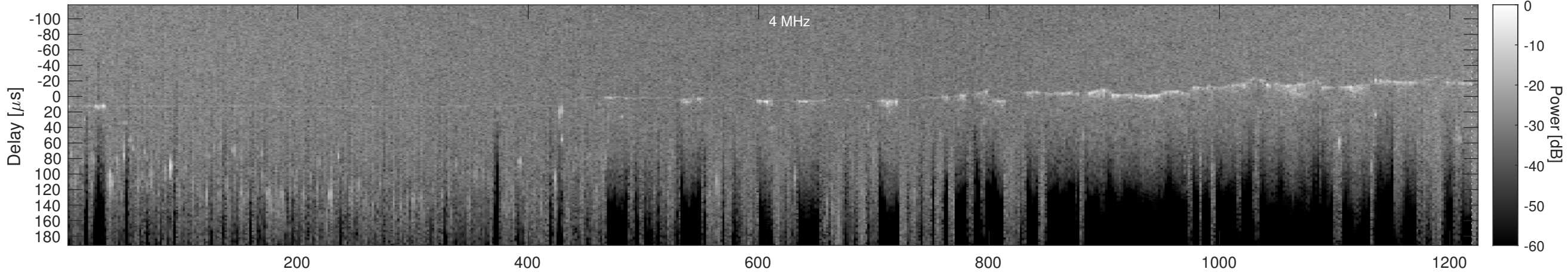
Orbit 5249, Cluttergram
