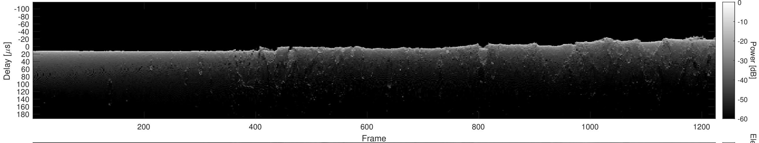
Orbit 5249, Cluttergram
