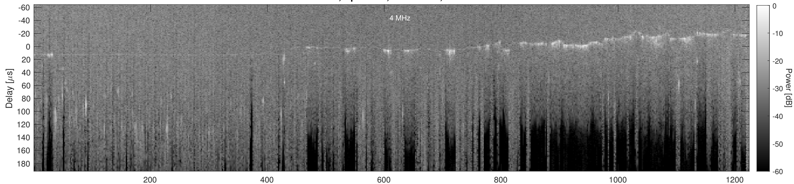
Orbit 5249, Cluttergram
