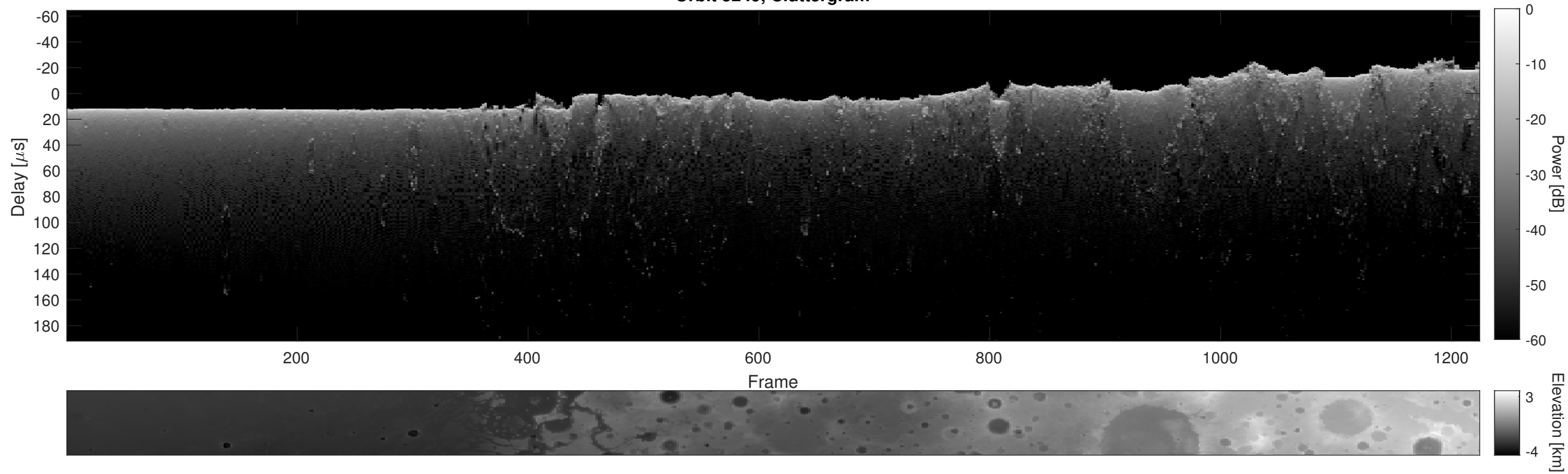
Orbit 5249, Cluttergram
