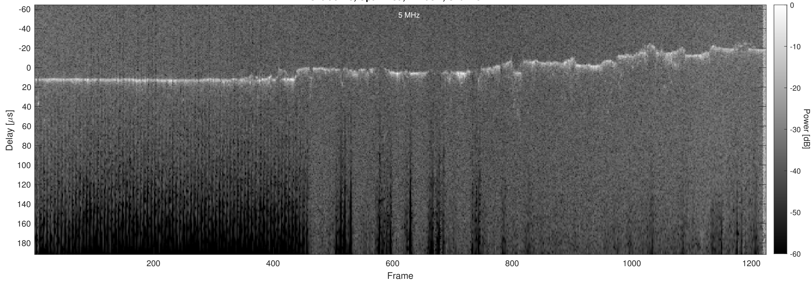
Orbit 5249, Optimized, Window, Channel 2
