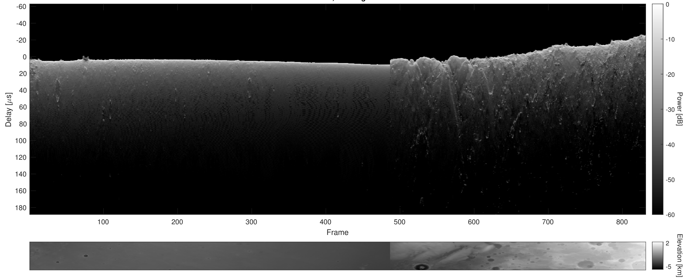
Orbit 5258, Cluttergram
