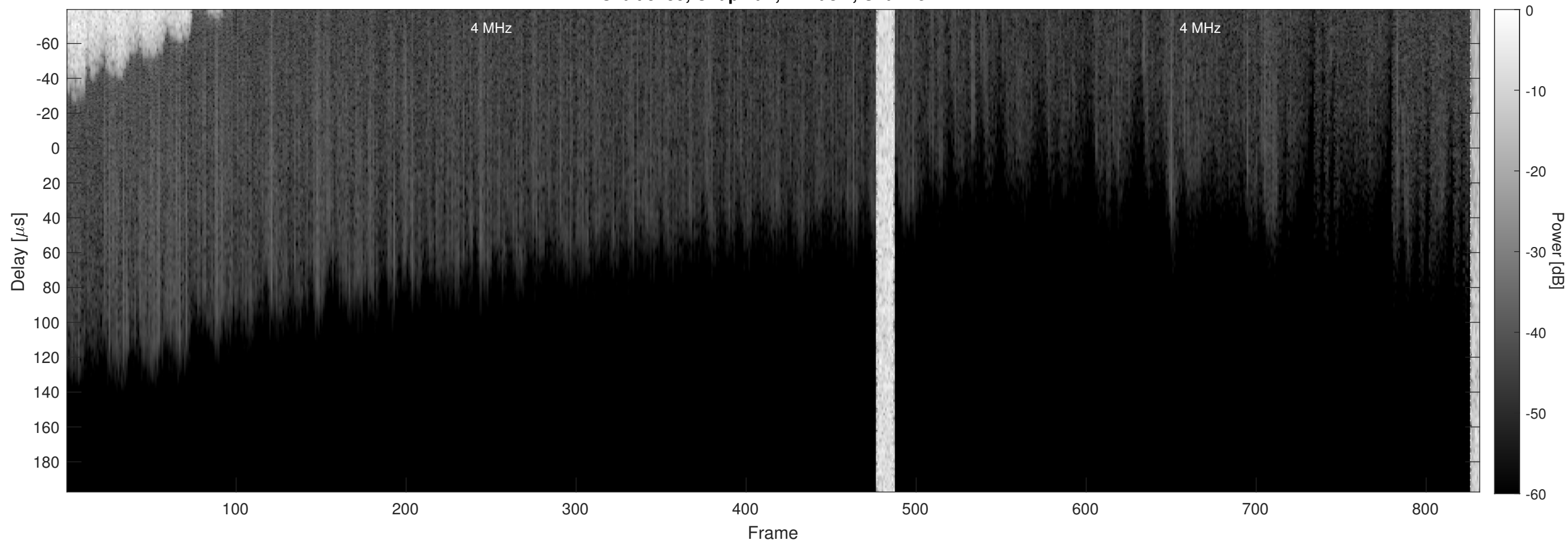
Orbit 5259, Chapman, Window, Channel 2
