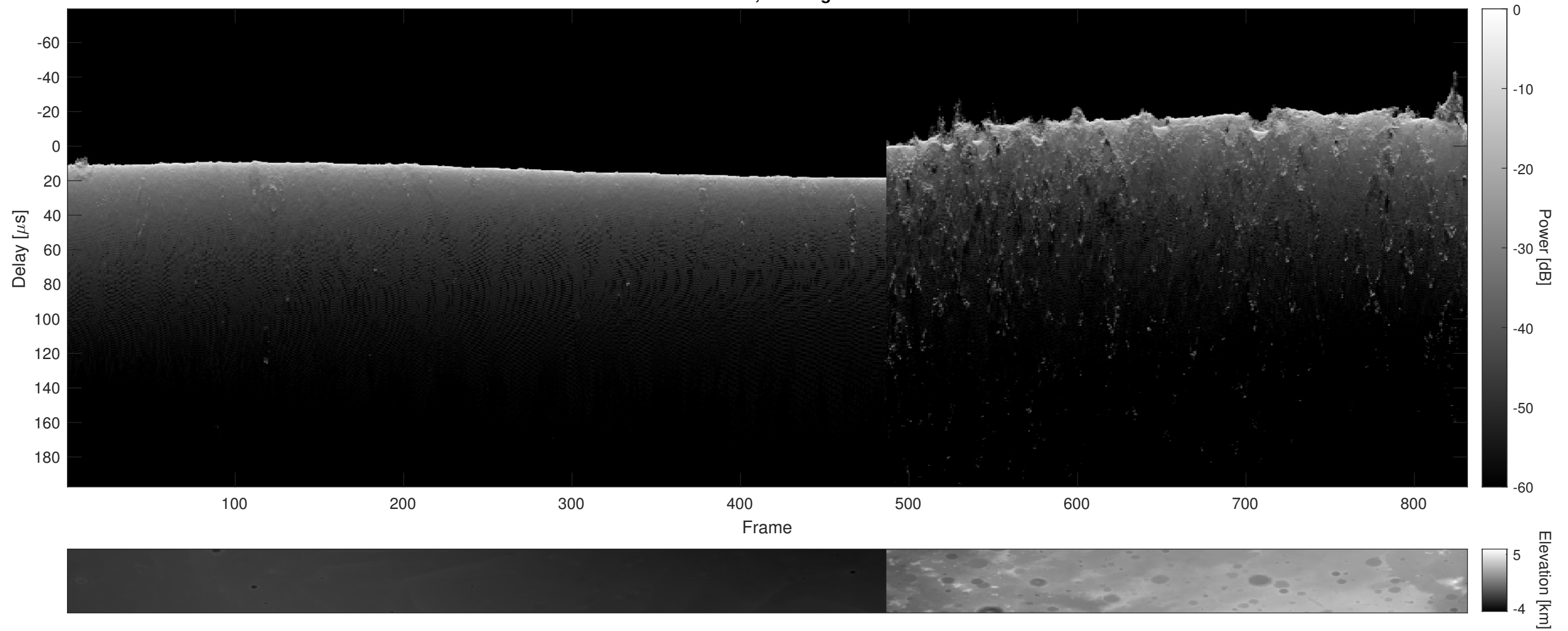
Orbit 5259, Cluttergram
