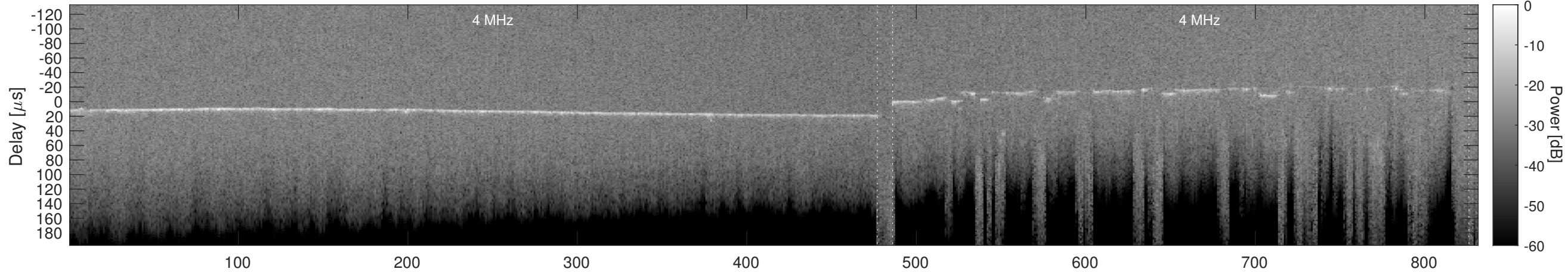
Orbit 5259, Cluttergram
