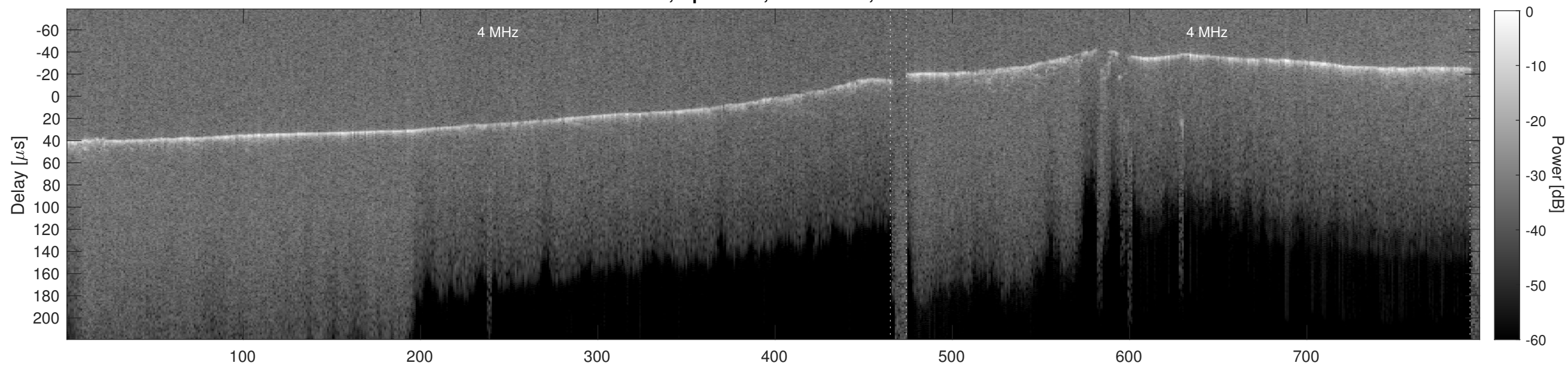
Orbit 5261, Cluttergram
