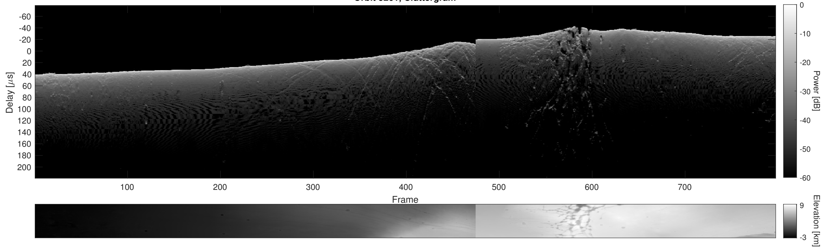
Orbit 5261, Cluttergram
