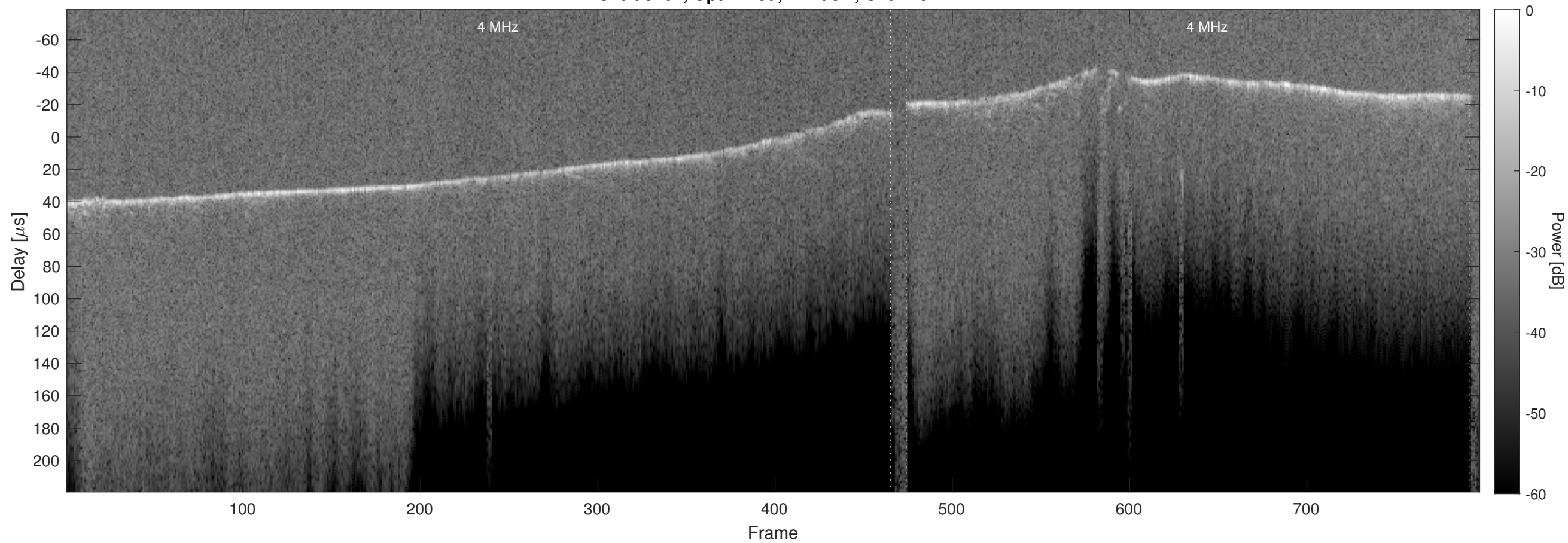
Orbit 5261, Optimized, Window, Channel 2
