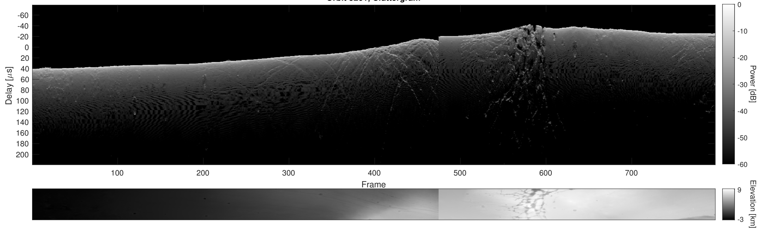
Orbit 5261, Cluttergram
