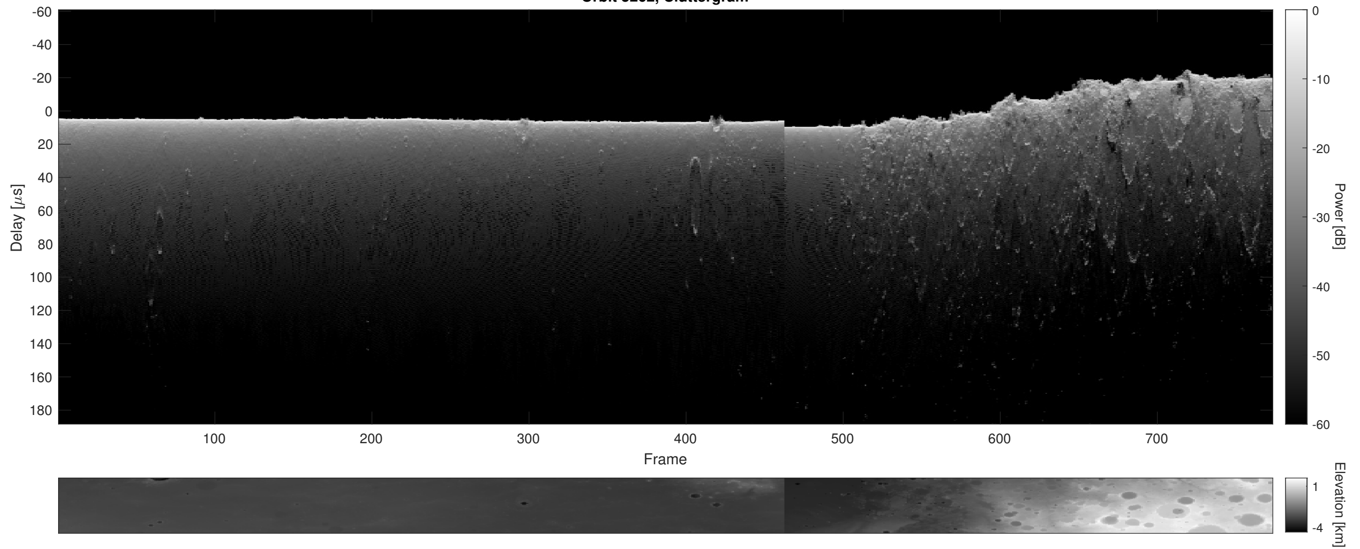
Orbit 5262, Cluttergram
