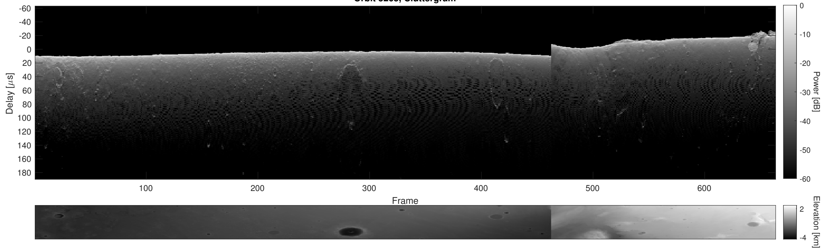
Orbit 5265, Cluttergram
