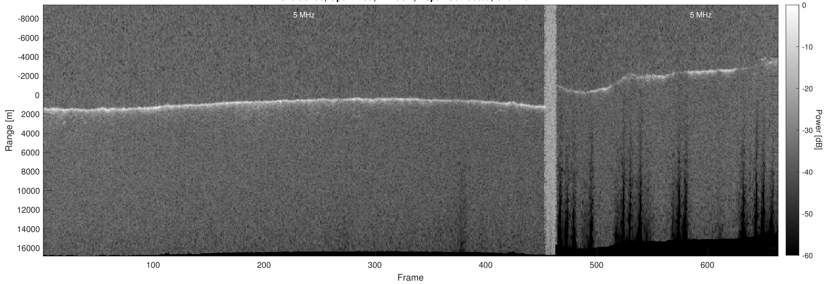
Orbit 5265, Optimized, Window, Depth-Corrected, Channel 2
