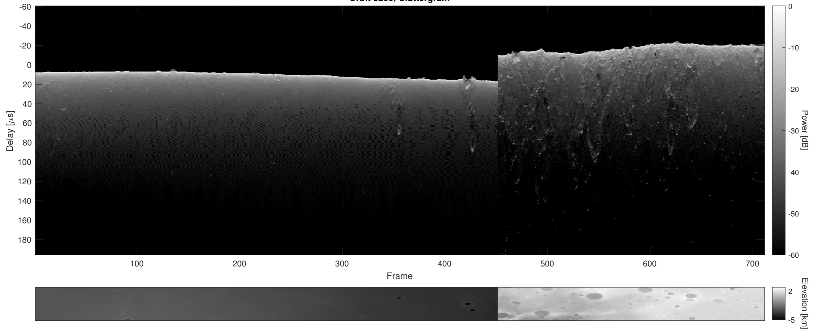
Orbit 5266, Cluttergram
