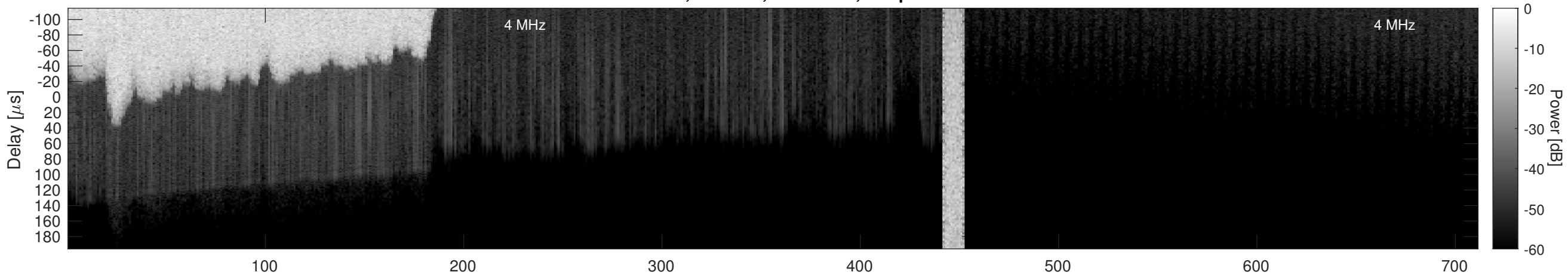
Orbit 5266, Window, Channel 2, Optimized
