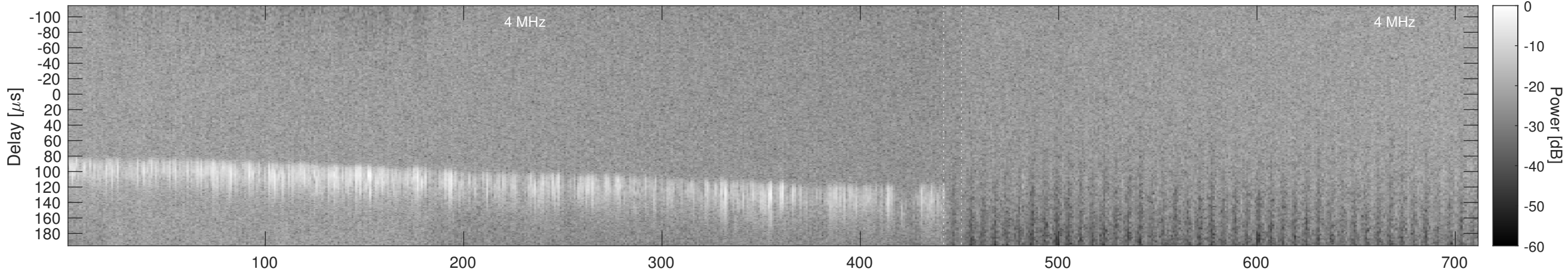
Orbit 5266, Window, Channel 2, Chapman
