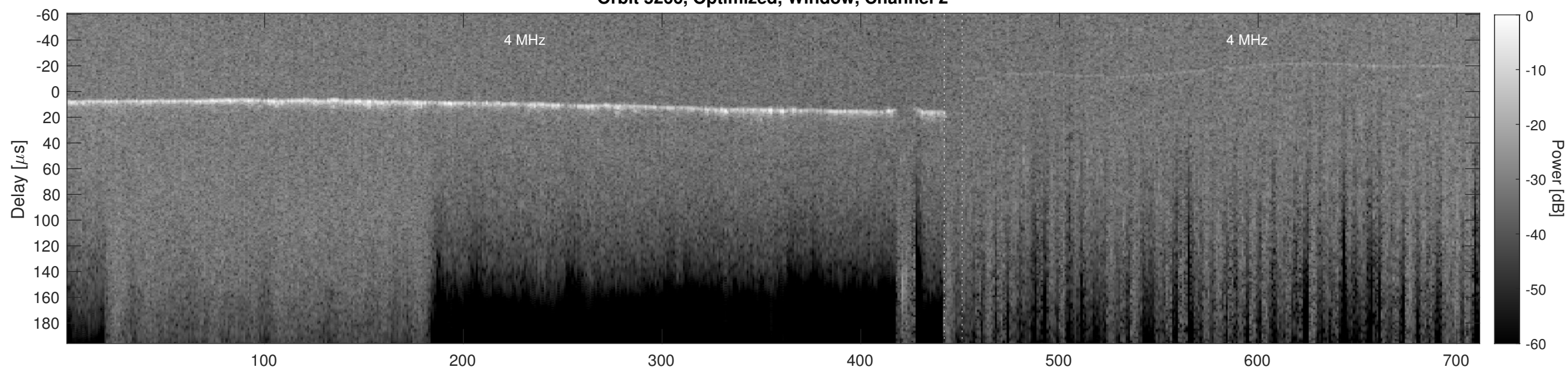
Orbit 5266, Cluttergram
