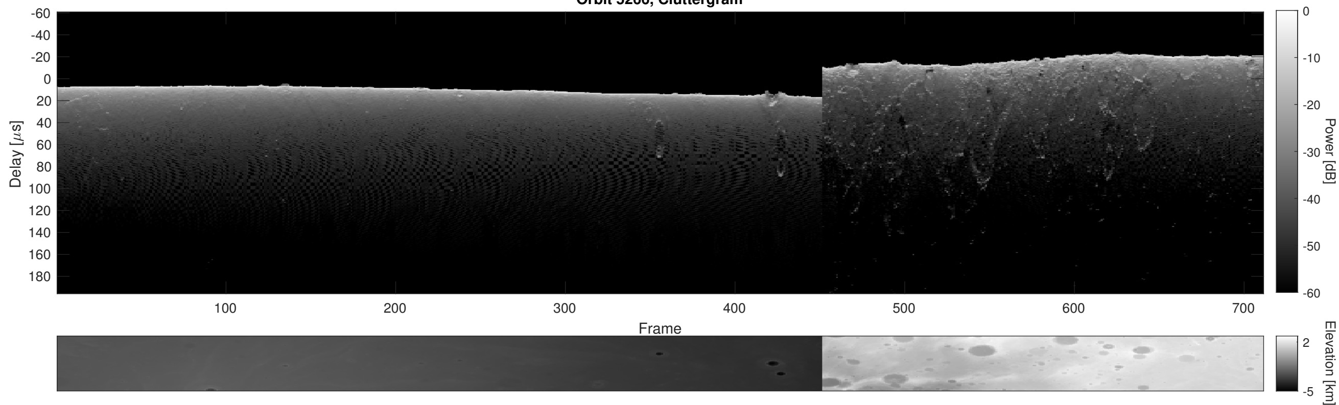
Orbit 5266, Cluttergram
