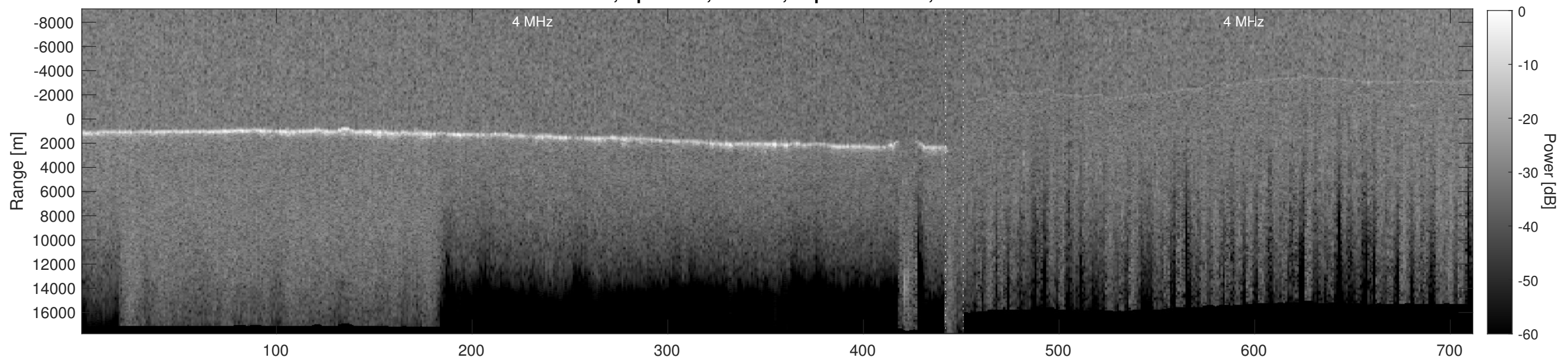
Orbit 5266, Depth-Corrected Cluttergram
