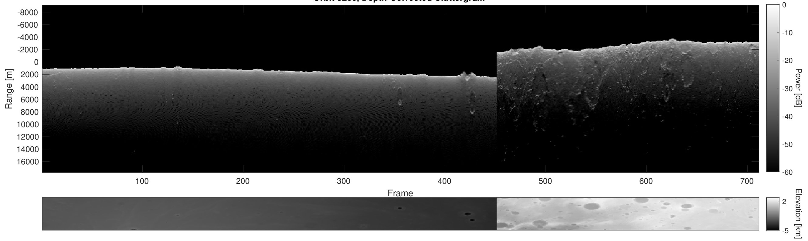
Orbit 5266, Depth-Corrected Cluttergram
