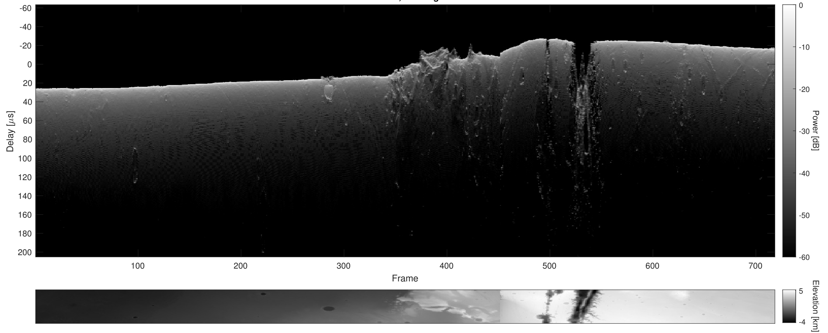
Orbit 5268, Cluttergram
