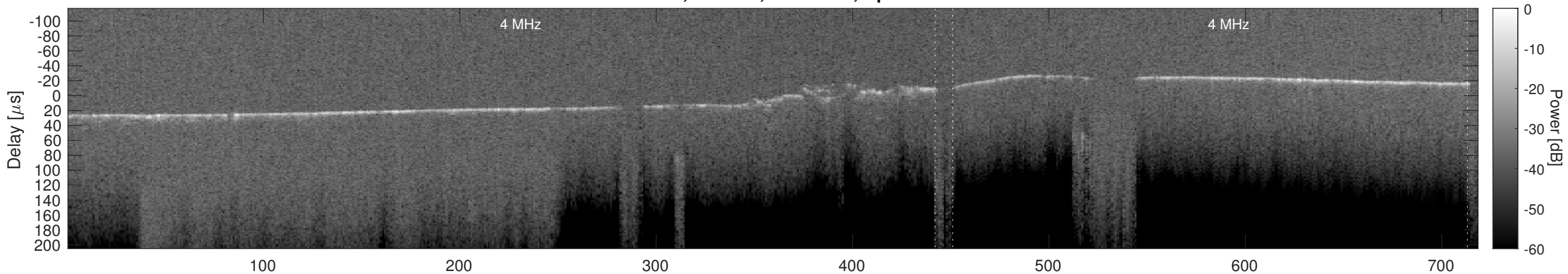
Orbit 5268, Cluttergram
