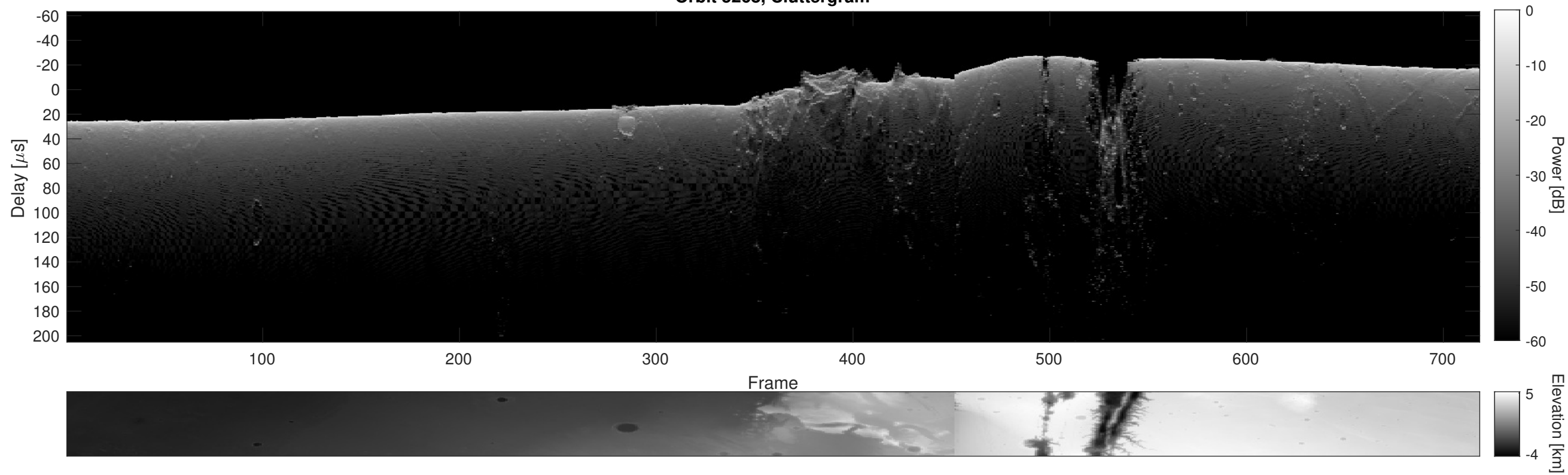
Orbit 5268, Cluttergram
