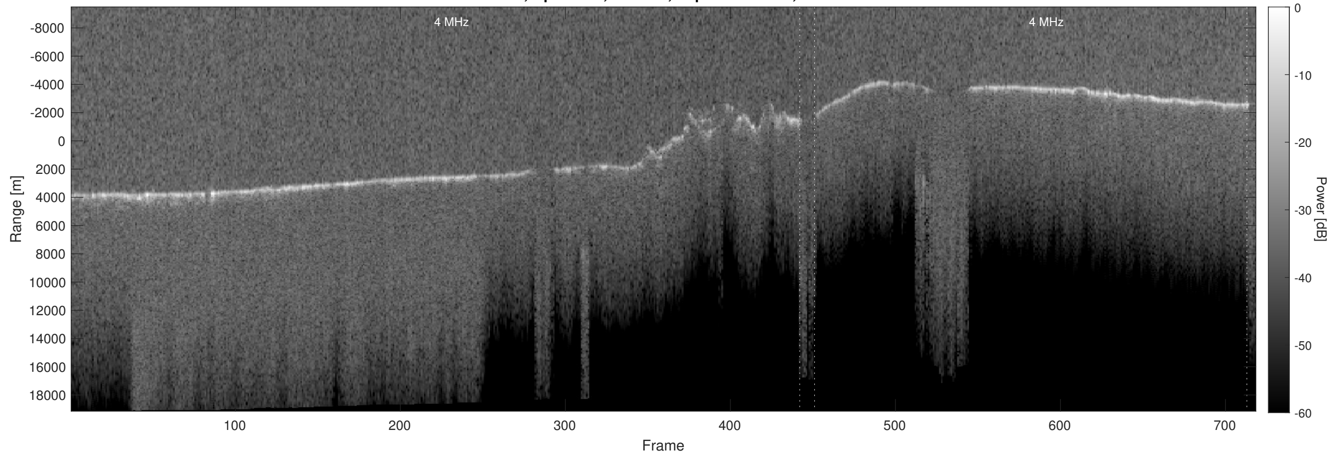
Orbit 5268, Optimized, Window, Depth-Corrected, Channel 2
