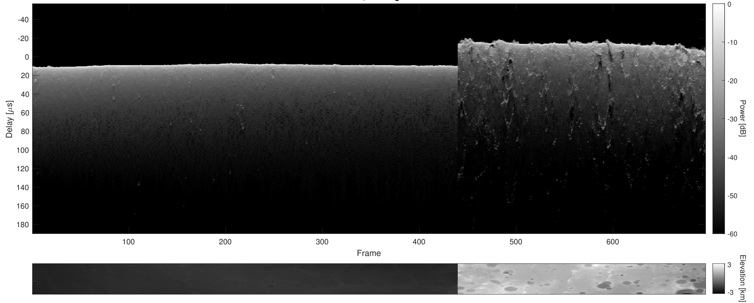
Orbit 5270, Cluttergram
