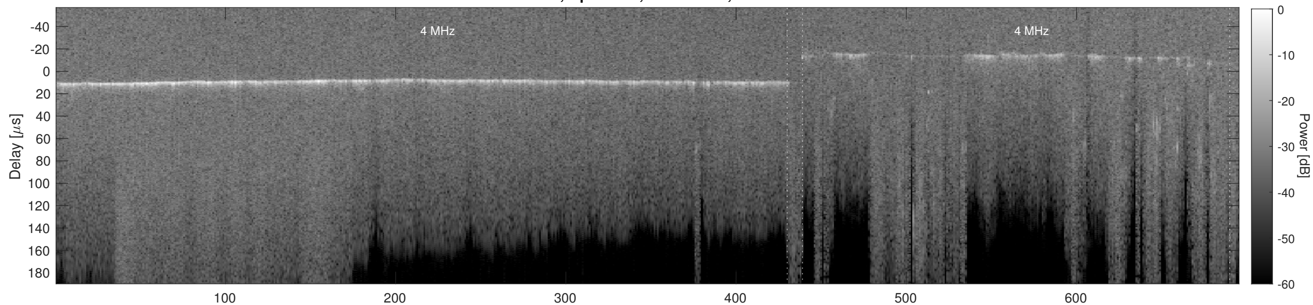
Orbit 5270, Cluttergram
