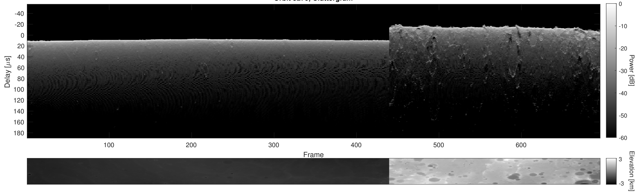
Orbit 5270, Cluttergram
