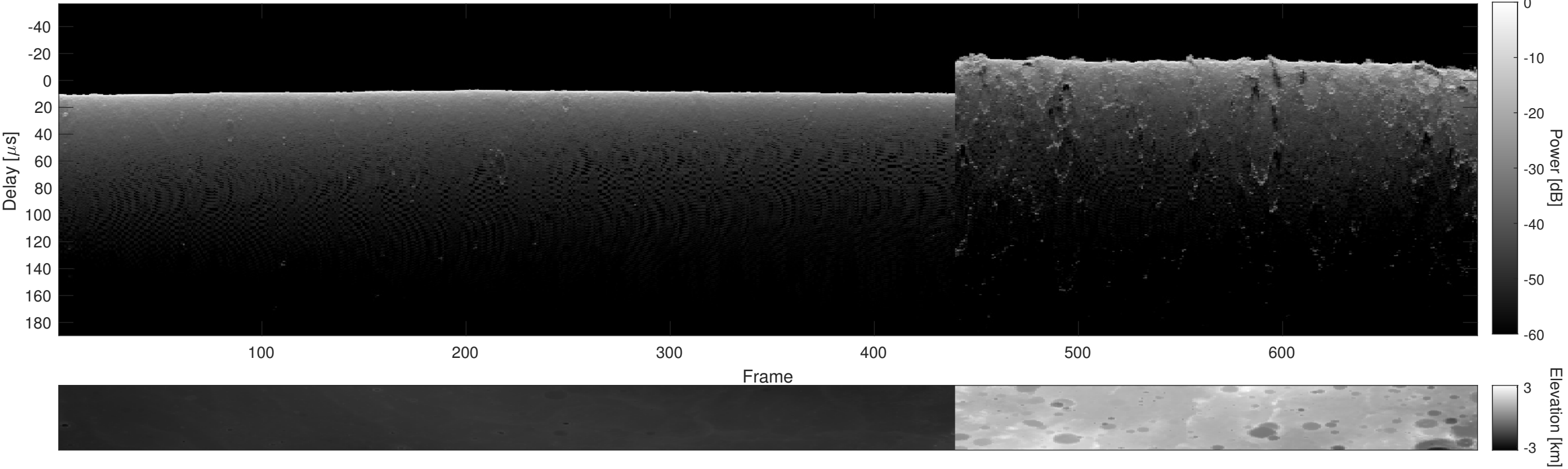
Orbit 5270, Cluttergram
