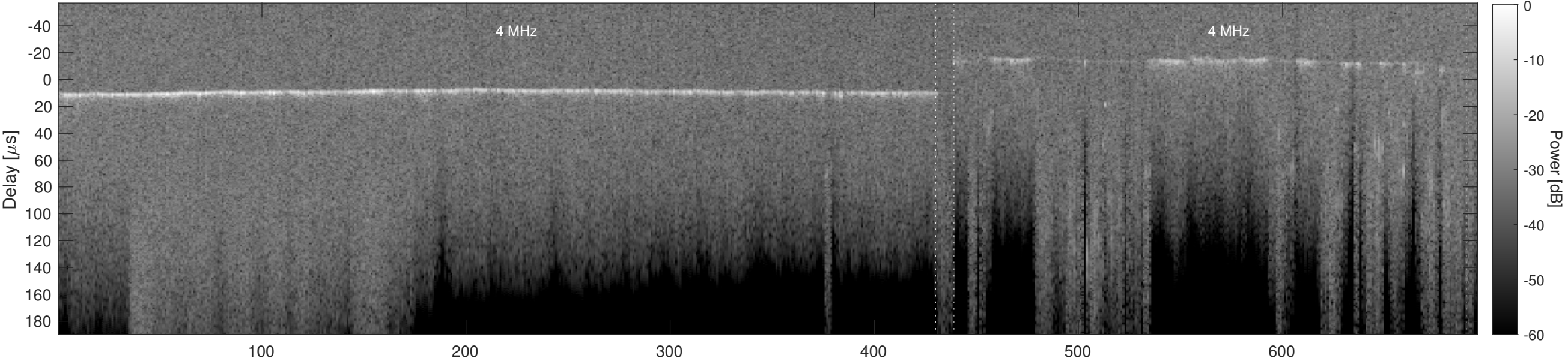
Orbit 5270, Cluttergram
