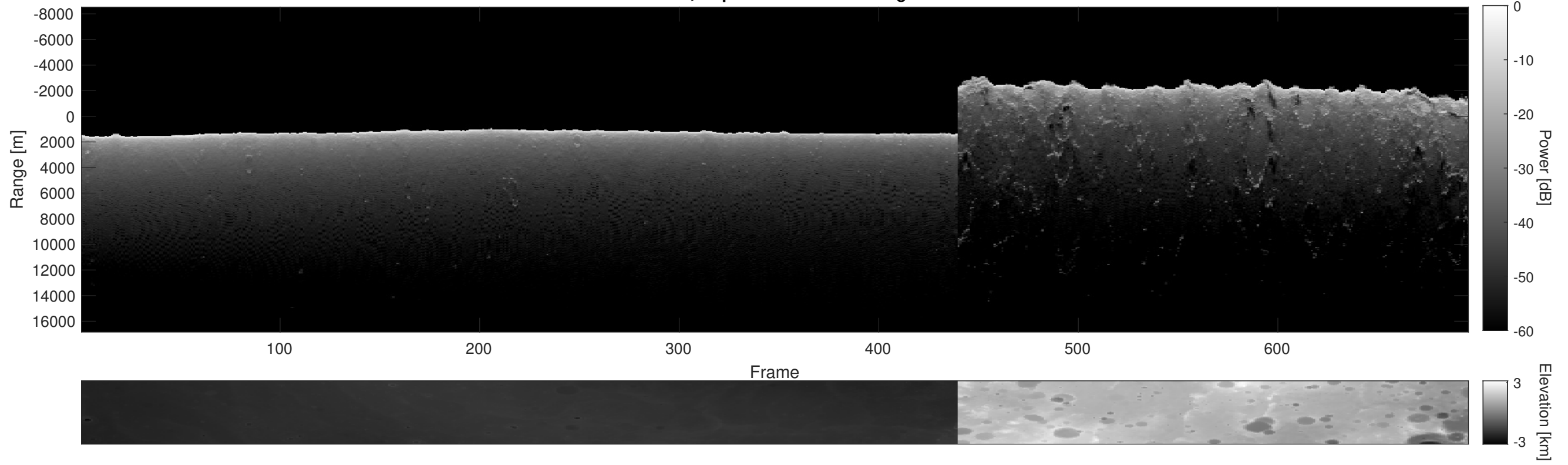
Orbit 5270, Depth-Corrected Cluttergram
