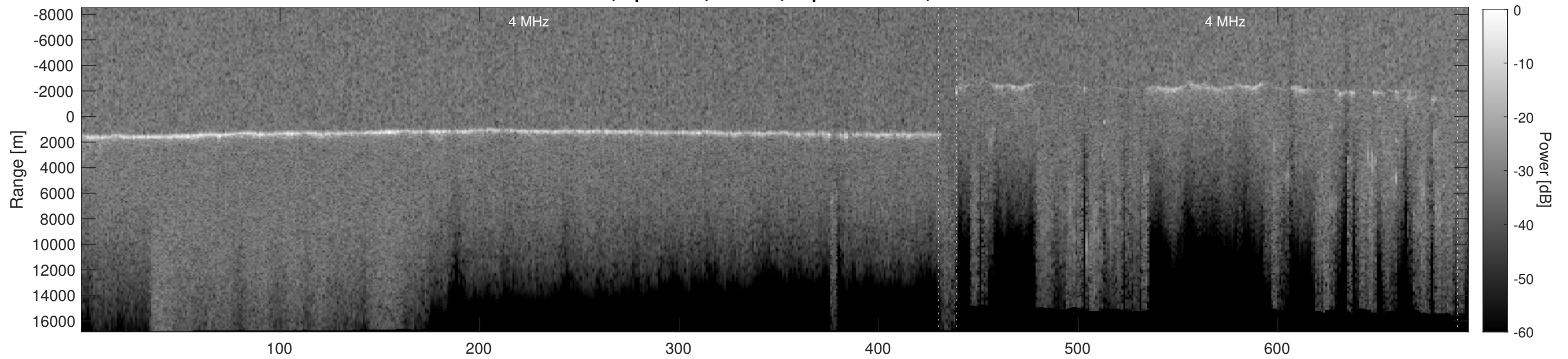
Orbit 5270, Depth-Corrected Cluttergram
