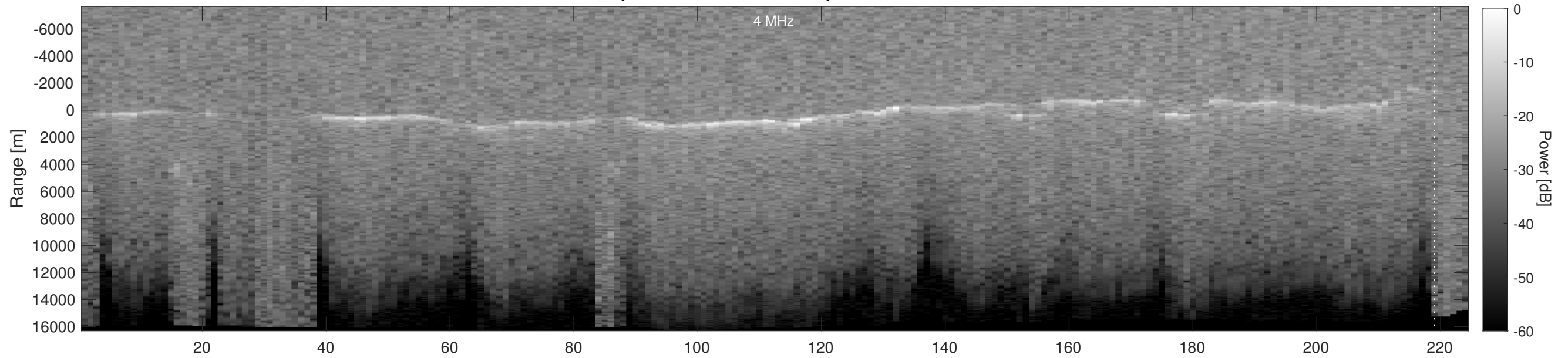
Orbit 5271, Depth-Corrected Cluttergram
