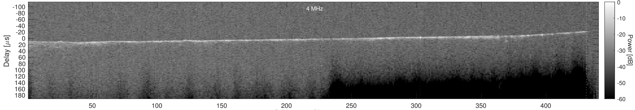
Orbit 5272, Cluttergram
