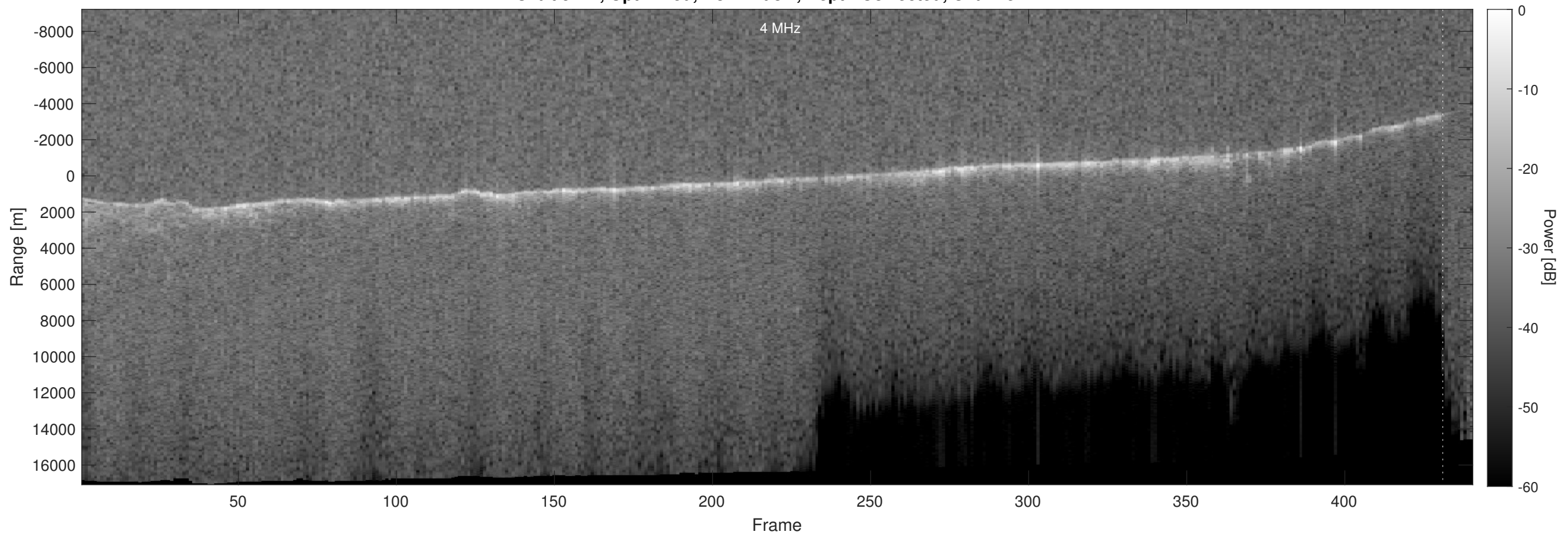
Orbit 5272, Optimized, No Window, Depth-Corrected, Channel 2
