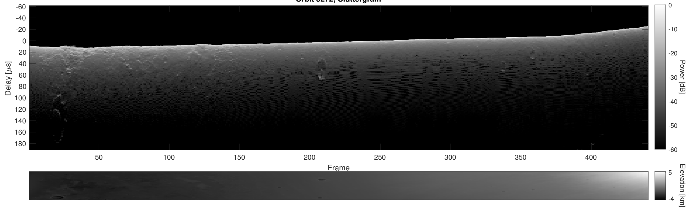
Orbit 5272, Cluttergram
