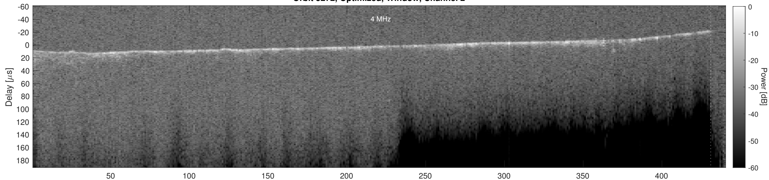
Orbit 5272, Cluttergram
