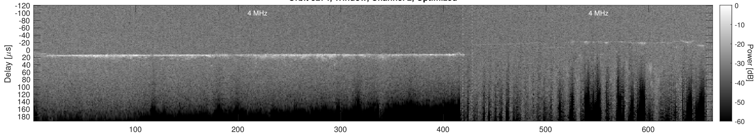
Orbit 5274, Cluttergram
