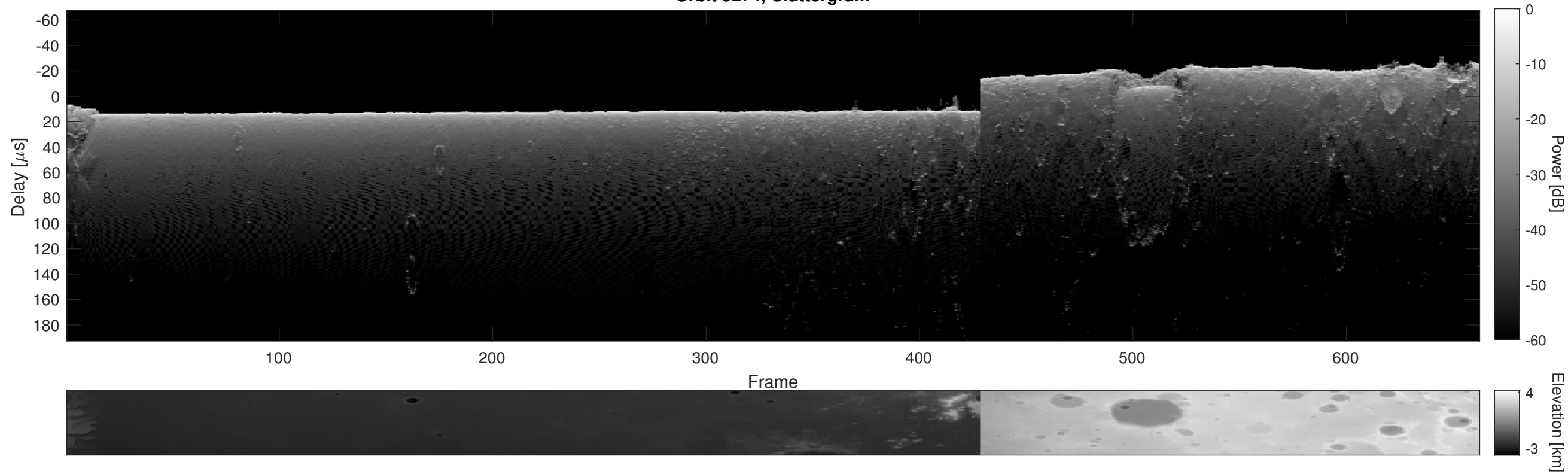
Orbit 5274, Cluttergram
