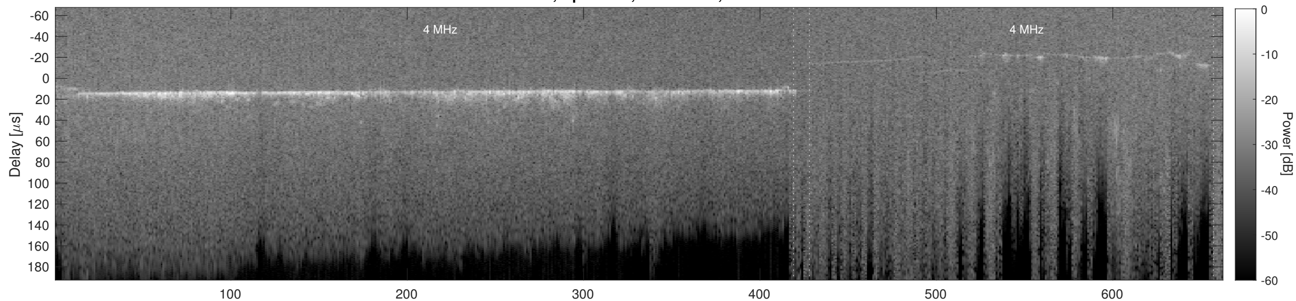
Orbit 5274, Cluttergram
