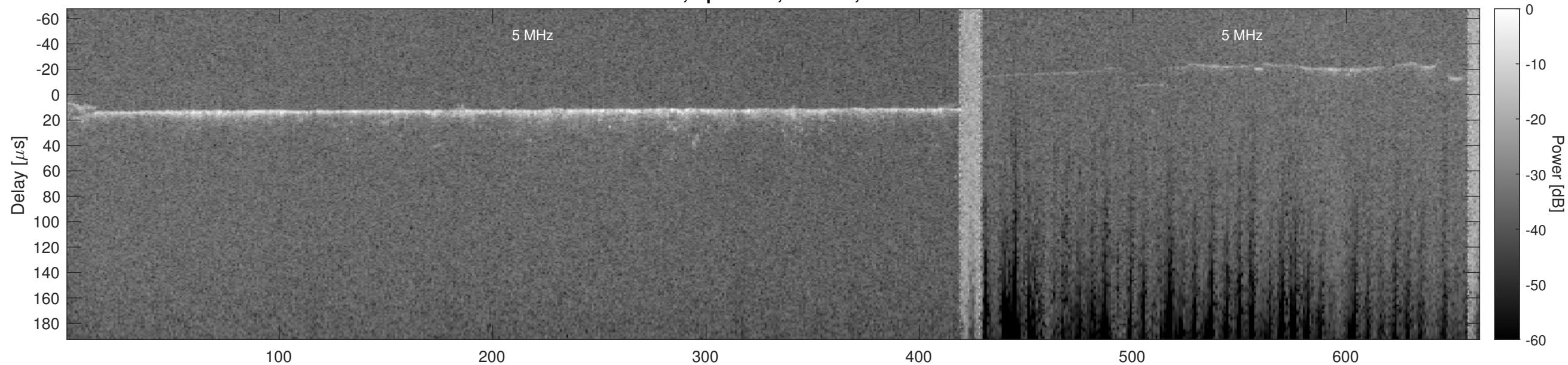
Orbit 5274, Optimized, Window, Channel 2
