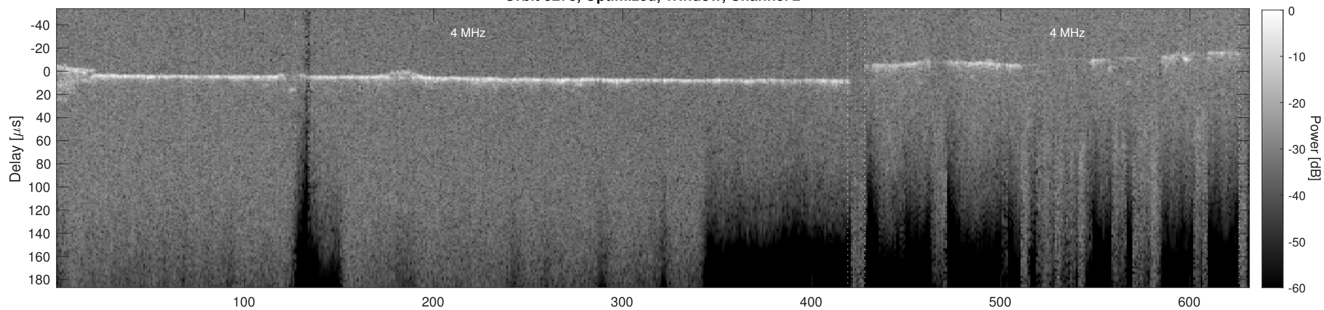
Orbit 5278, Cluttergram
