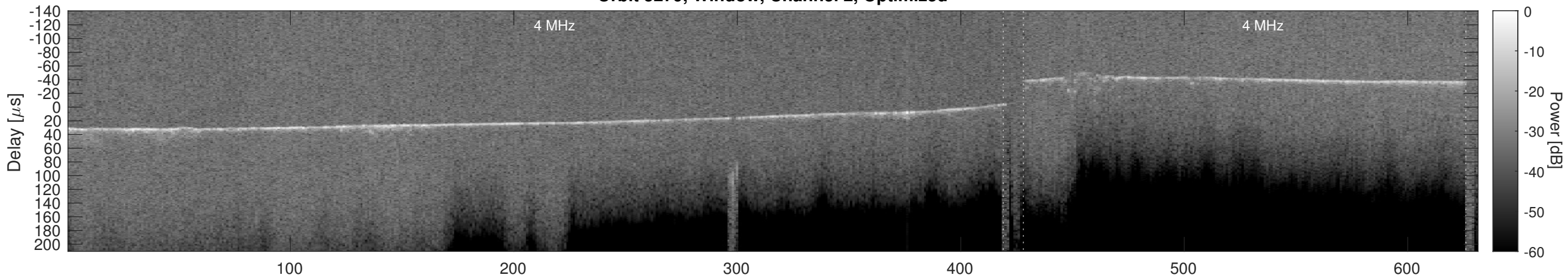
Orbit 5279, Cluttergram
