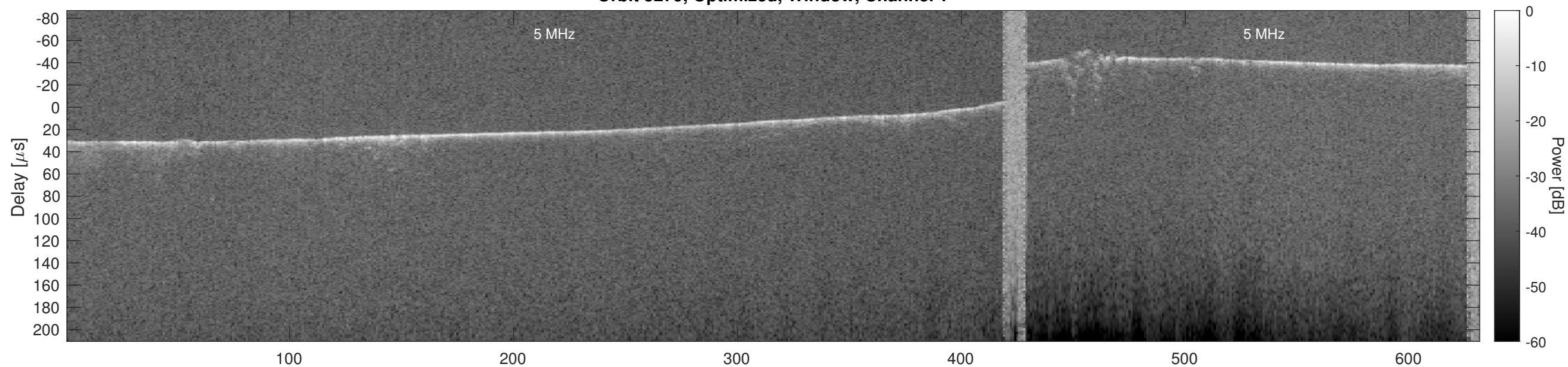
Orbit 5279, Optimized, Window, Channel 2
