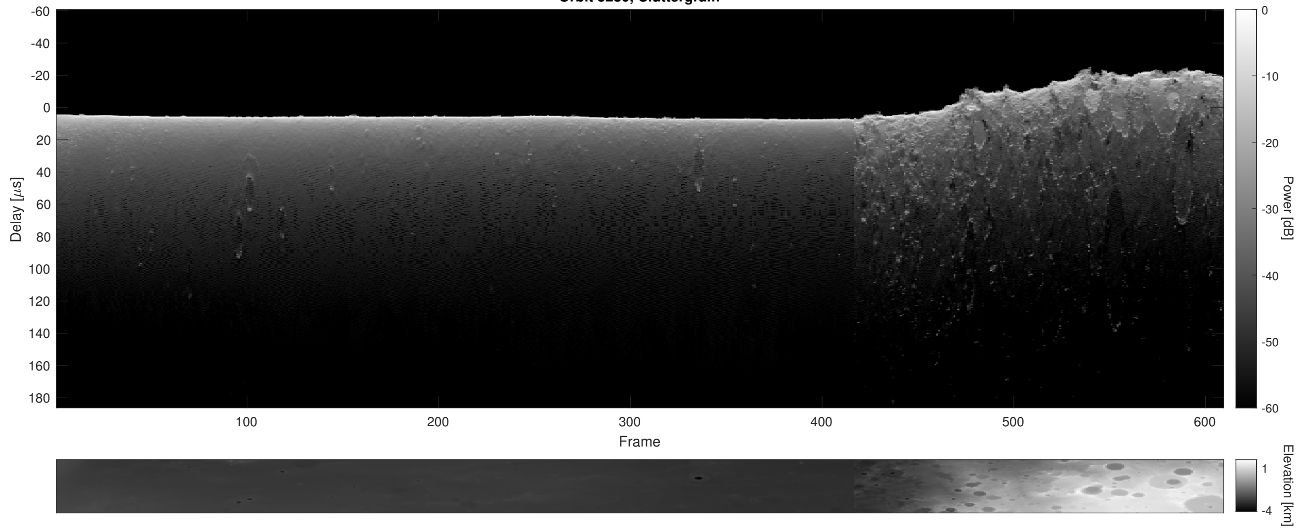
Orbit 5280, Cluttergram
