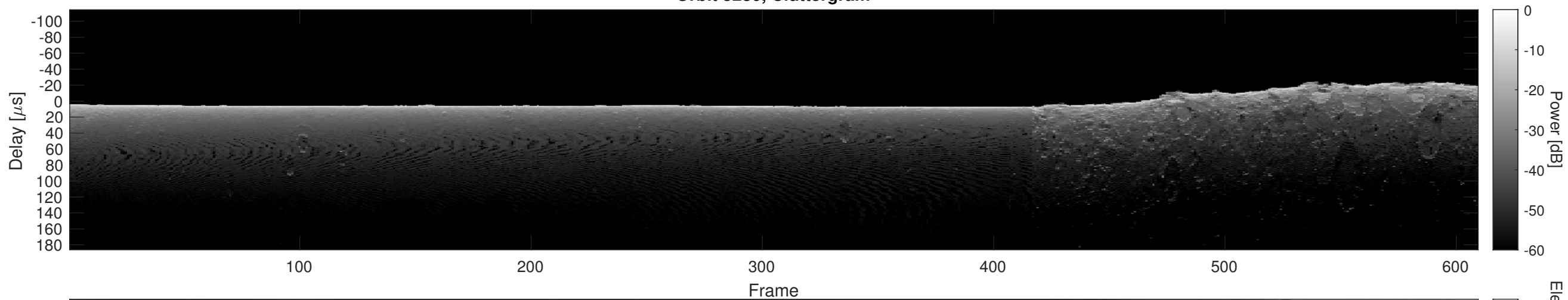
Orbit 5280, Cluttergram
