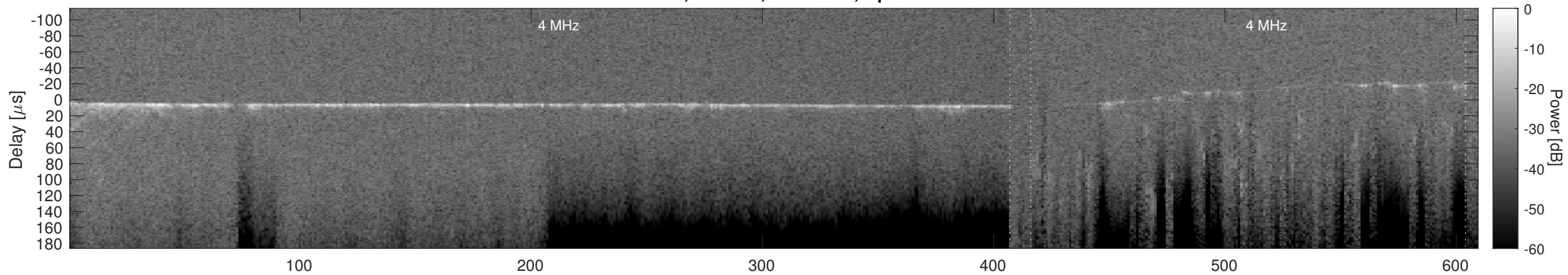
Orbit 5280, Cluttergram
