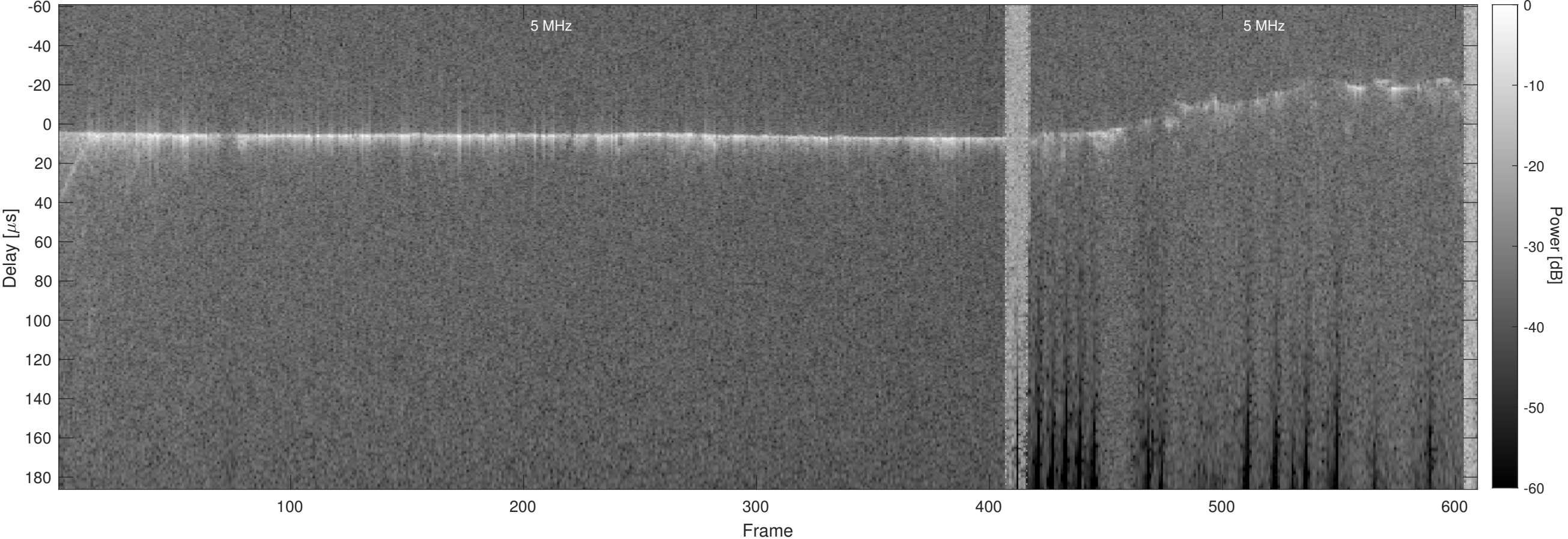
Orbit 5280, Optimized, No Window, Channel 2
