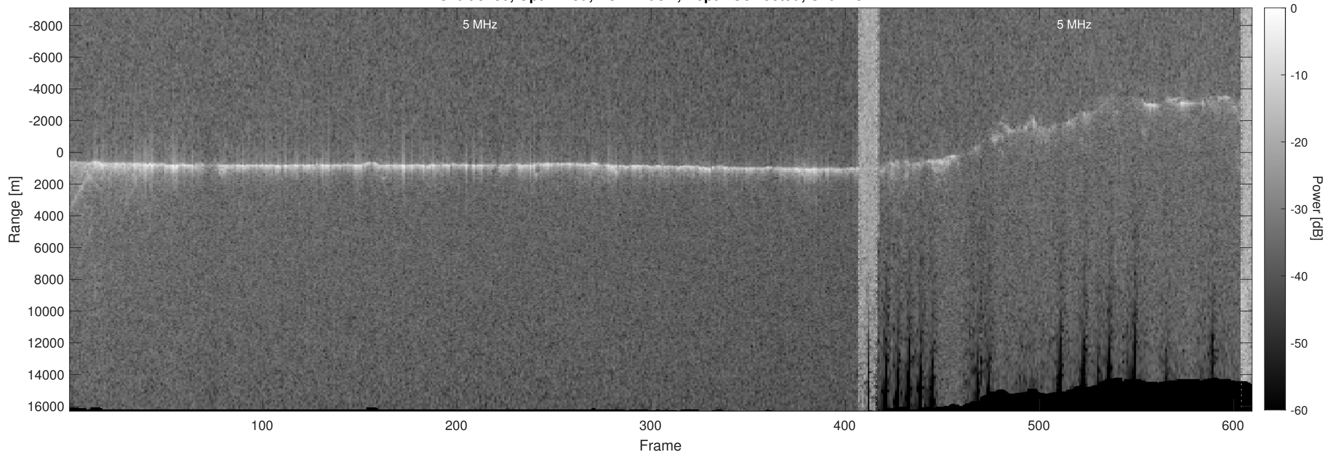
Orbit 5280, Optimized, No Window, Depth-Corrected, Channel 2
