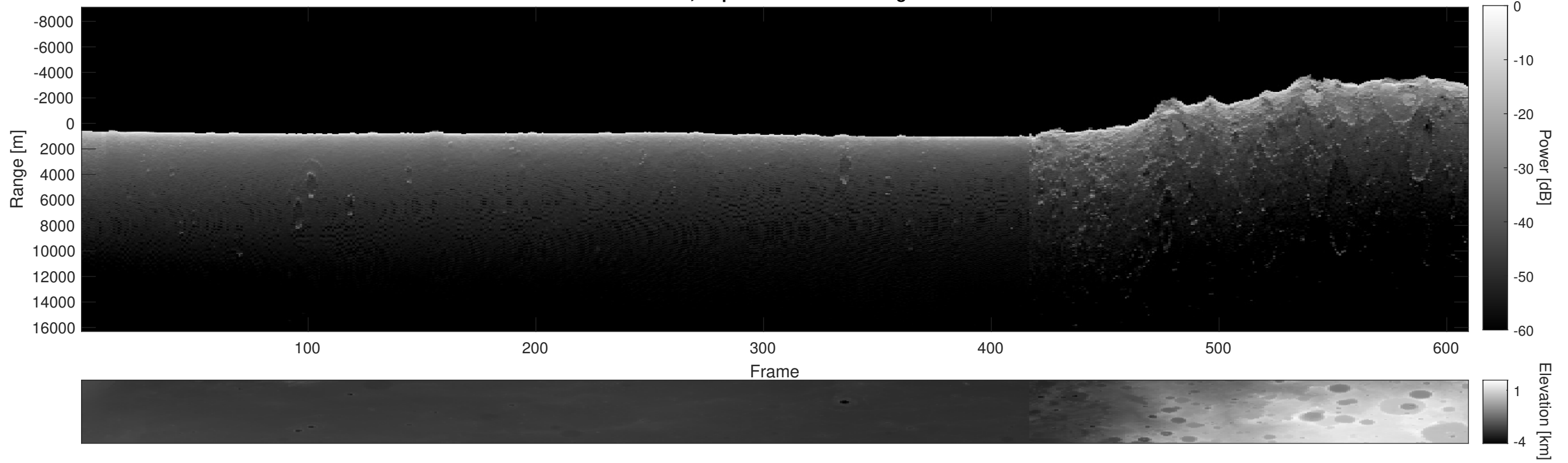
Orbit 5280, Depth-Corrected Cluttergram
