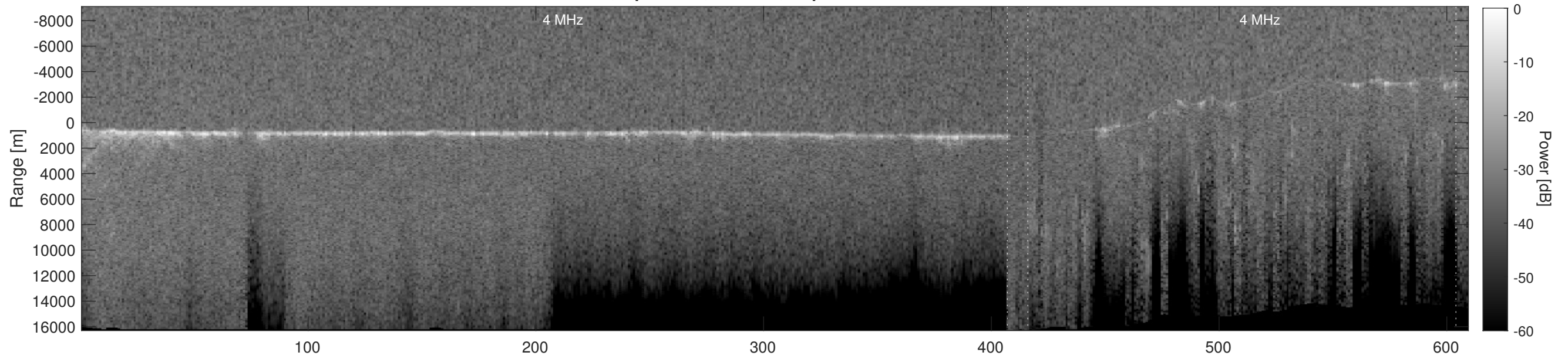
Orbit 5280, Depth-Corrected Cluttergram
